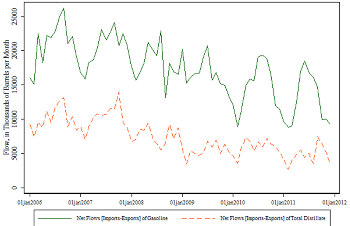
Figure 6: PADD 2 net flows of gasoline and distillate (diesel)
