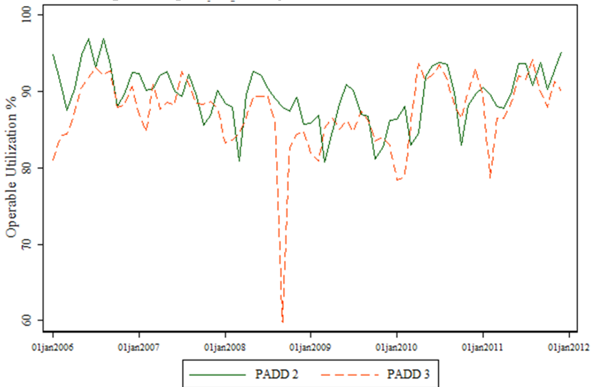
Figure 8: Operable refinery utilization in PADDs 2 and 3
