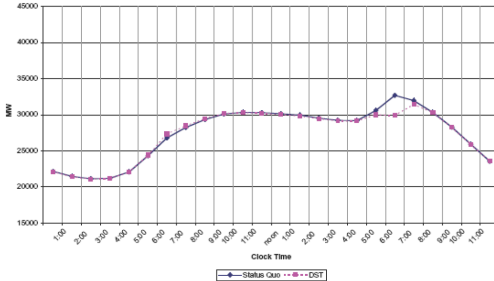
Figure 9: Simulation of DST in California, March 1998-2000 (CEC, 2001)
