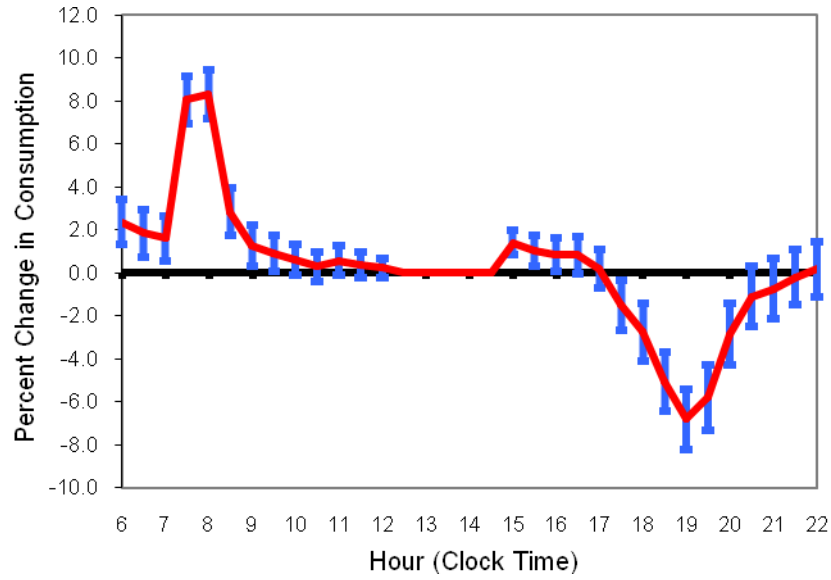
Figure 7: Half-hourly effects of extending DST on electricity use
